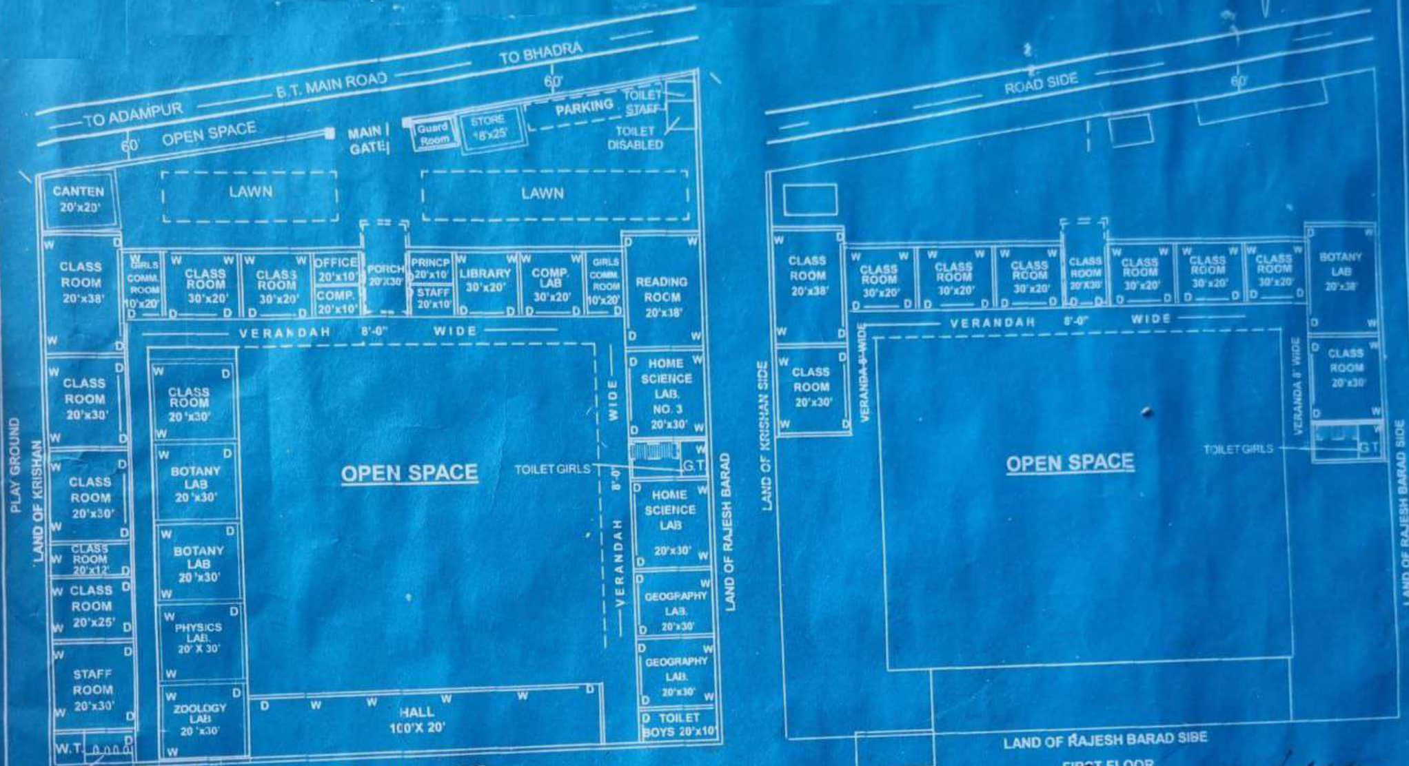
LAND OF RAJESH BARAD GROUND FLOOR
